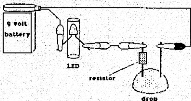
Figure 3: Conductivity Tester.
