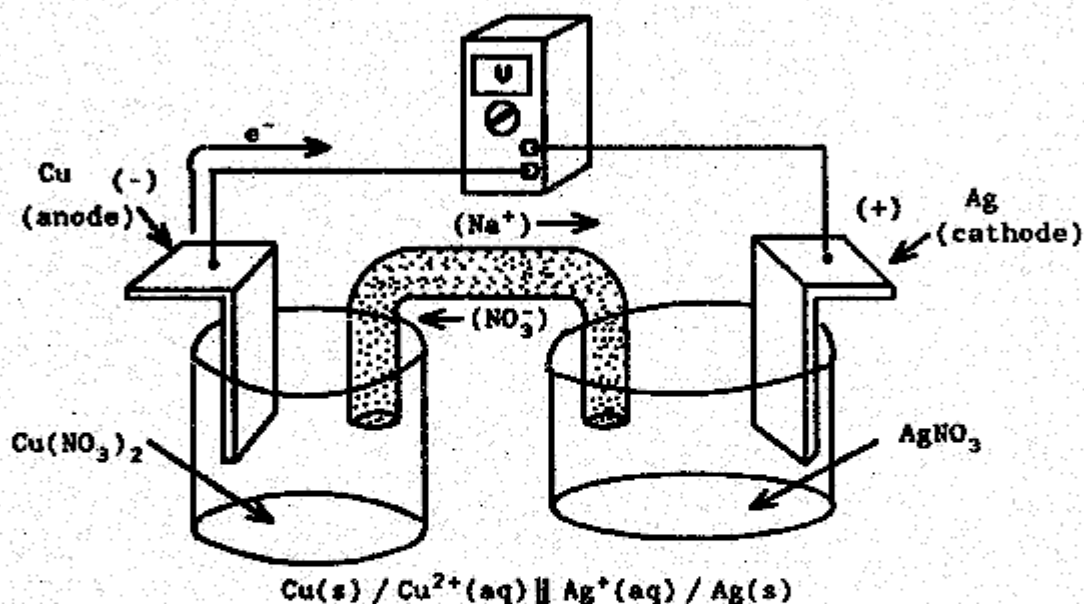
Voltaic Cell
